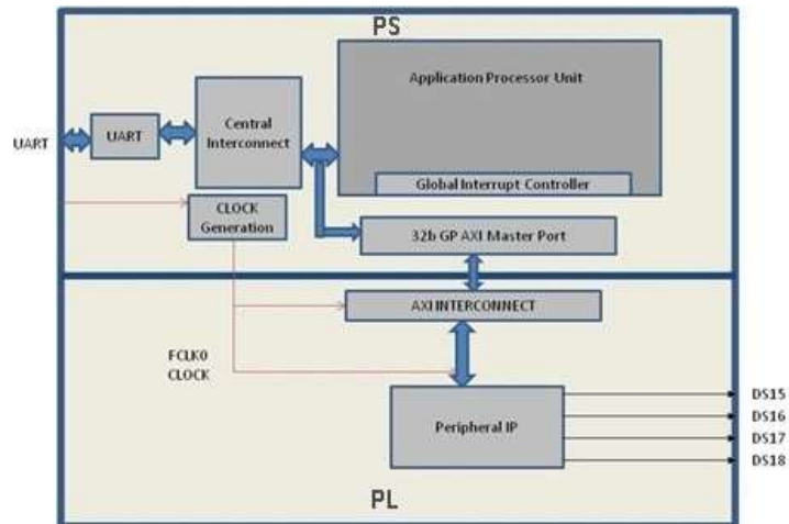
Figure 7-5: Block Diagram
