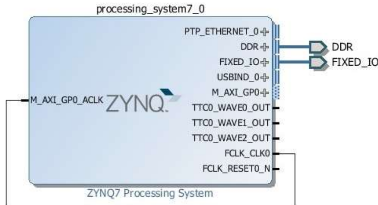
Figure 2-8: ZYNQ7 Processing System with Connection
