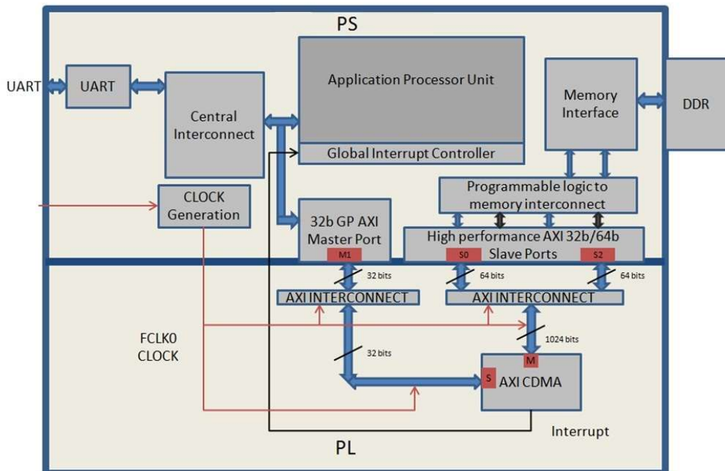
Figure 5-1: Block Diagram
