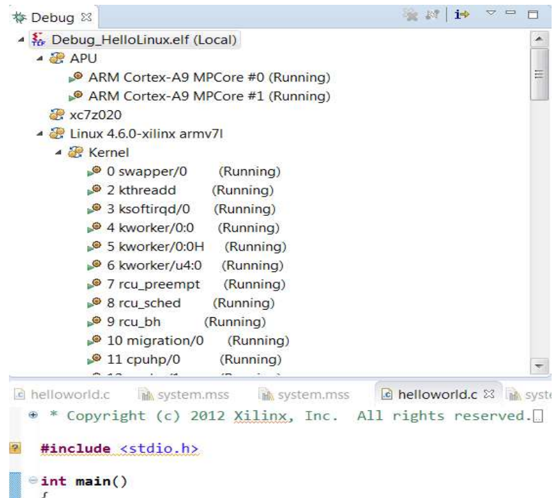
Figure 9-5: Debug Perspective
