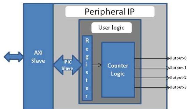
Figure 7-1: Block Diagram for Peripheral IP
