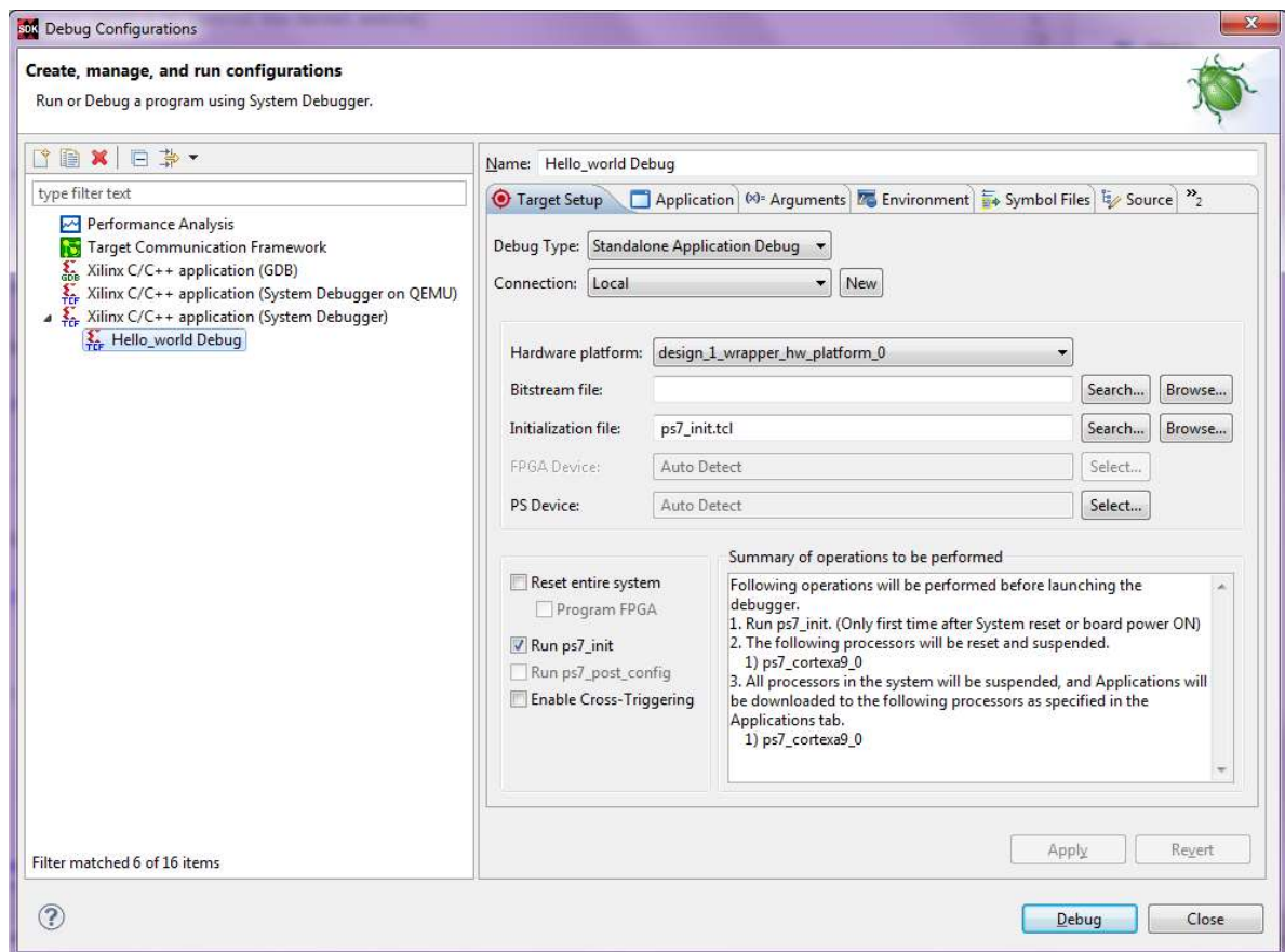
Figure 4-2: Debug Configurations
