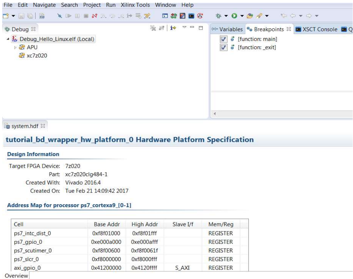
Figure 9-3: Debug Perspective
